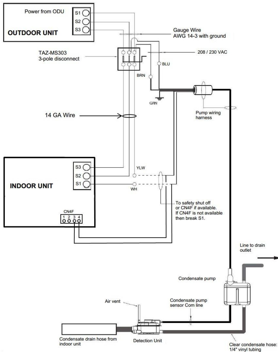
Figure 1. X87-721 or Si-30-230V Wiring Diagram
