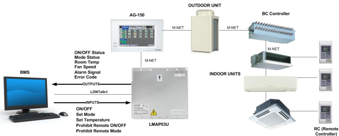
Figure 1. Typical CITY MULTI® control with LonWorks®
